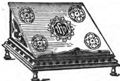
MISSAL STAND.
